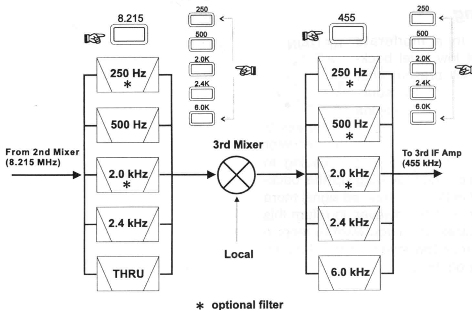
Main Receiver (VFO-A) IF Bandwidth Filter Selections
