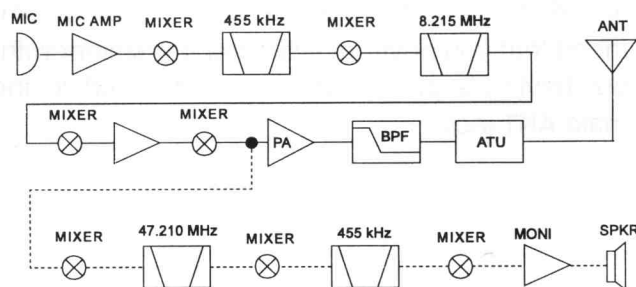
Monitor Circuit
