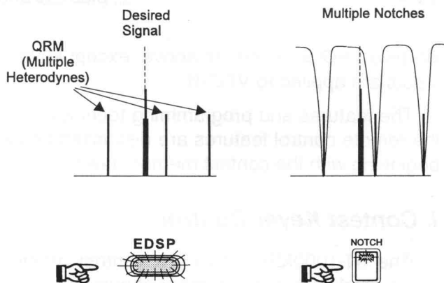
EDSP Auto Multiple Notch Action
