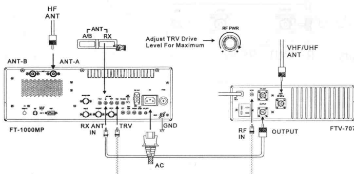
Example of Transverter Station Interconnections
